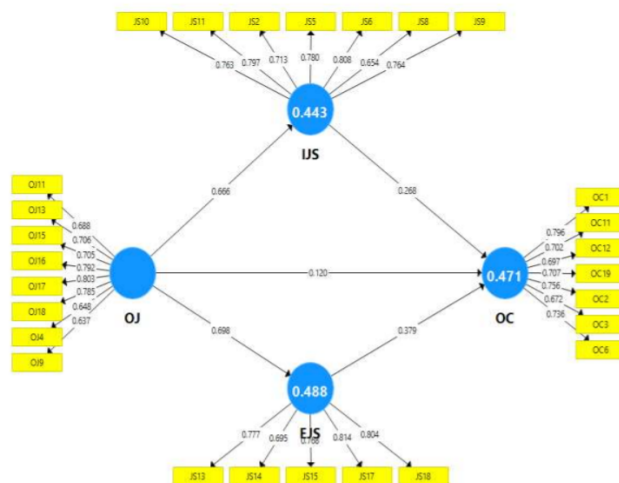
Figure 2. Model Fit
